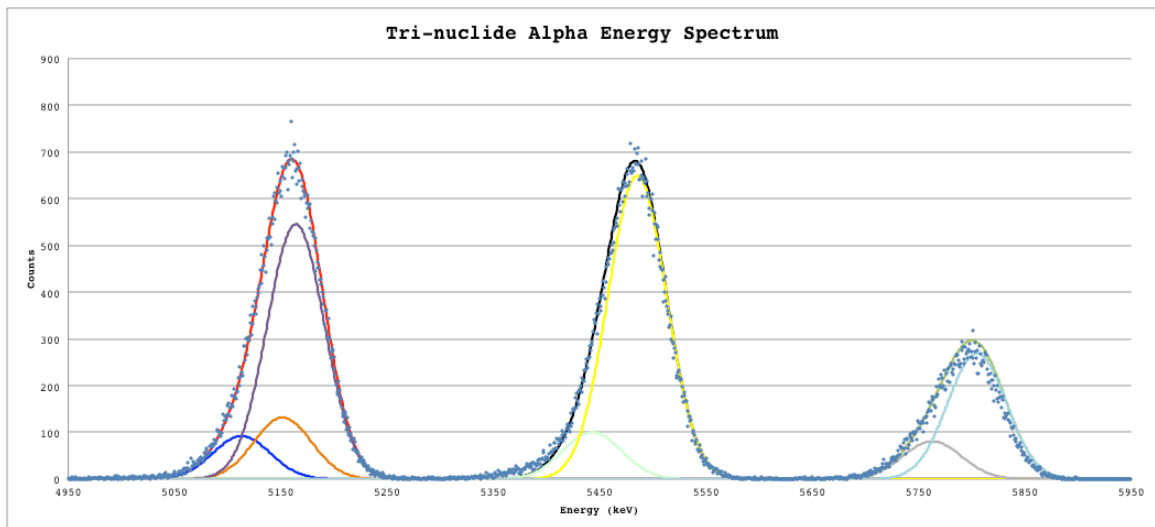
Figure 39 – Tri-nuclide alpha energy resolution spectrum
