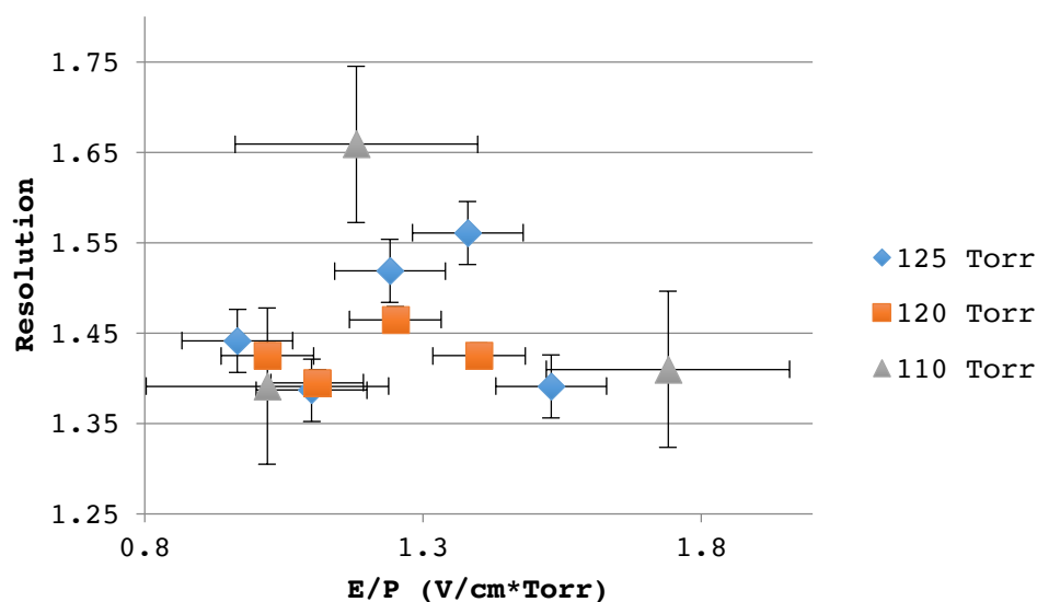
Figure 35 – ^{252}\text{Cf} alpha energy resolution vs. E/P for SiN window and isobutane gas at various pressures
